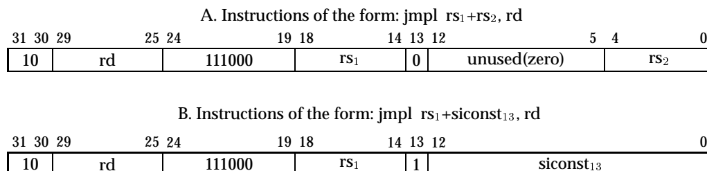
Figure 10.2 Instruction formats for jmpl instructions
